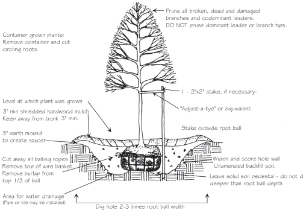
Tree Planting Detail
